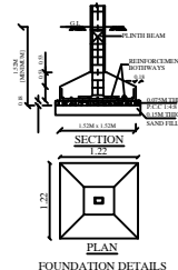
FOUNDATION DETAILS
