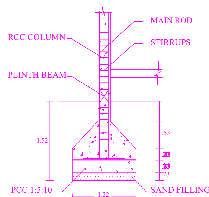
COLUMN DETAILS
