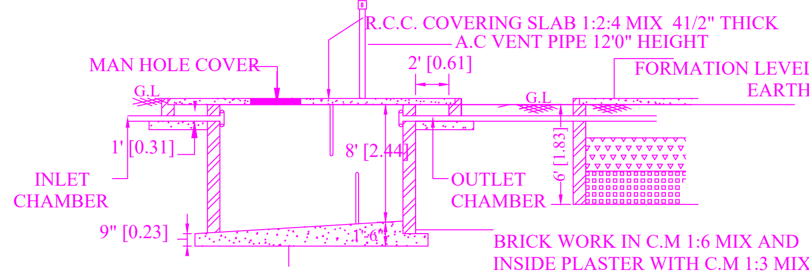
SEPTIC TANK
