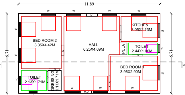
PROPOSED GROUND FLOOR
