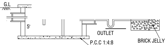
SECTION-AB
