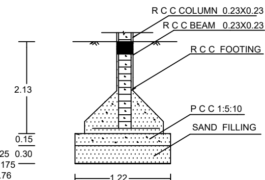
FOUNDATION DETAILS
