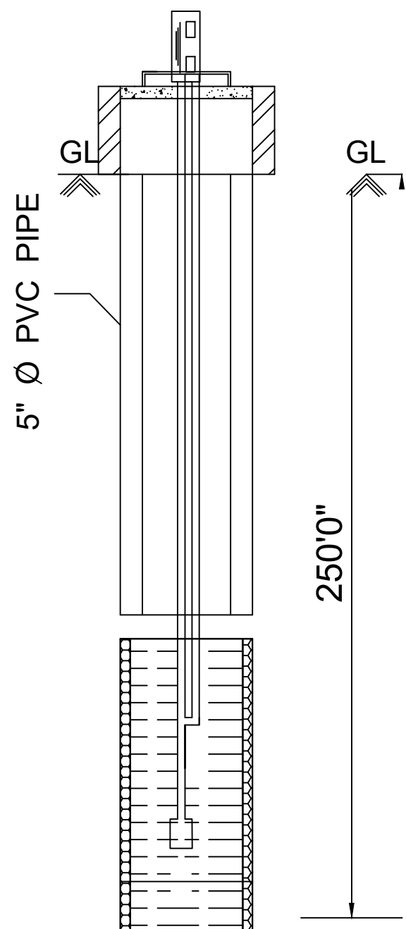
BOREWELL DETAILS
