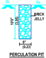
PERCOLATION PIT
