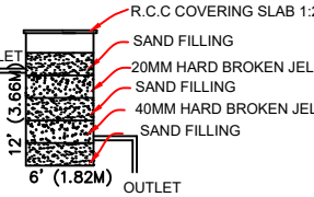
Bath & wash basin pipe line connection is directly connected to the rectangle pit for recycling the waste water. WATER_TANK_CAPACITY_L=4200LTRS
