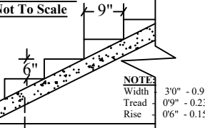
Staircase Detail
