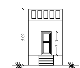
FRONT ELEVATION
