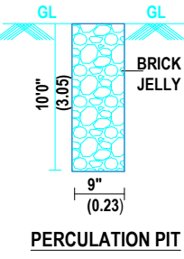
PERCOLATION PIT
