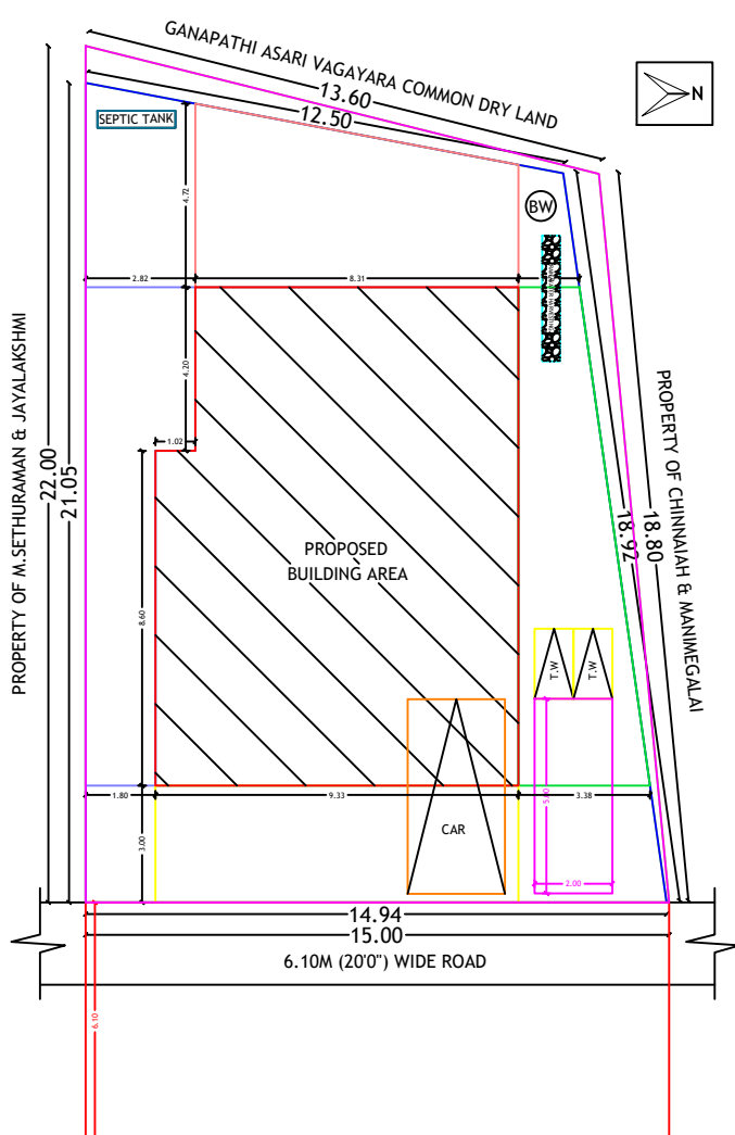
SITE PLAN
