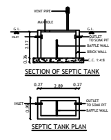
SECTION OF SEPTIC TANK
