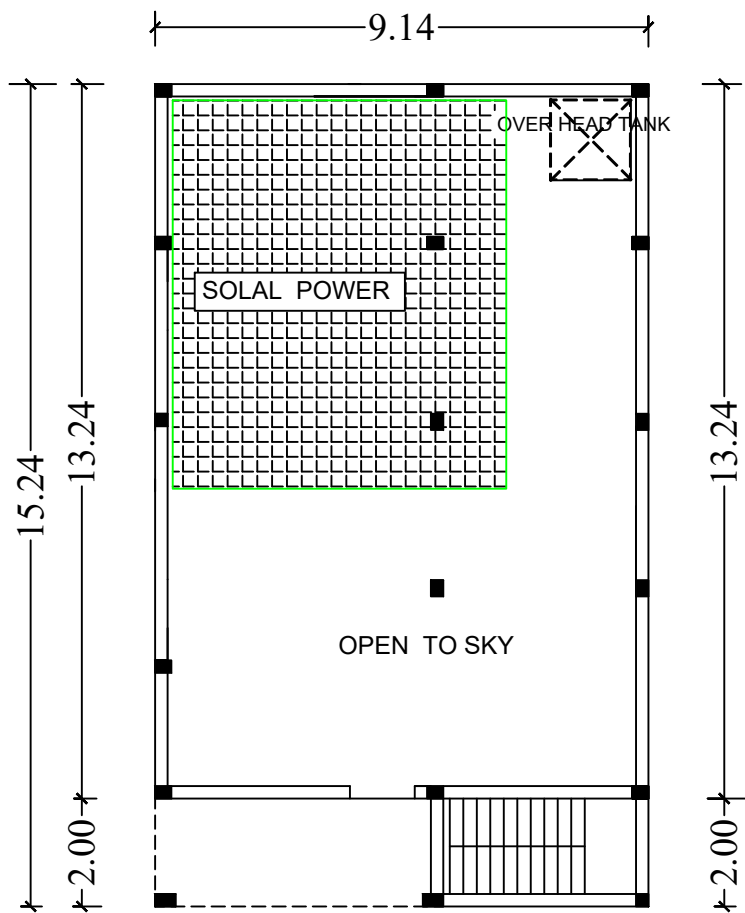
TERRACE FLOOR
