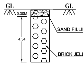
DETAILS OF RAINWATER HARVESTING TANK.(NTS)
