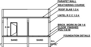
SECTION ON "A B"
