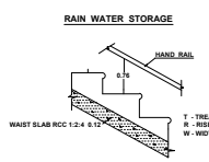
RAIN WATER STORAGE
