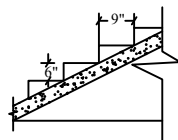
STAIR CASE DETAILS
