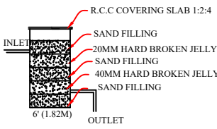
RAIN WATER HARVESTING SYSTEM
