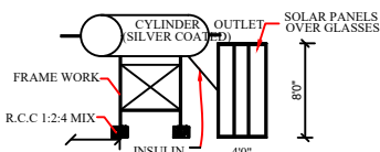
SOLAR HEATING SYSTEM
