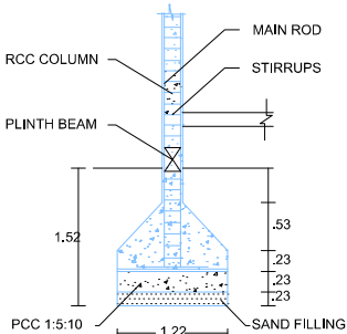
COLUMN DETAILS
