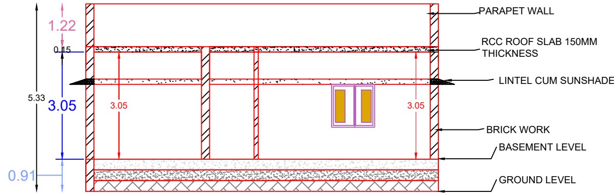
SECTION ON A-B (SCALE 1:150)
