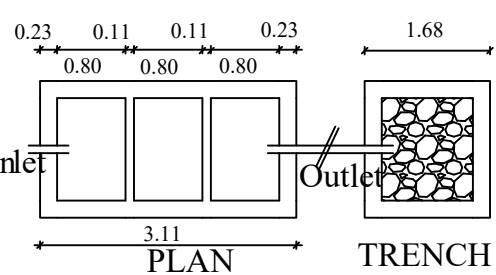
( U trap septic tank design to be used )
