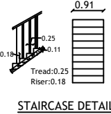
STAIRCASE DETAIL
