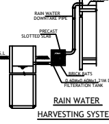
RAIN WATER HARVESTING SYSTEM
