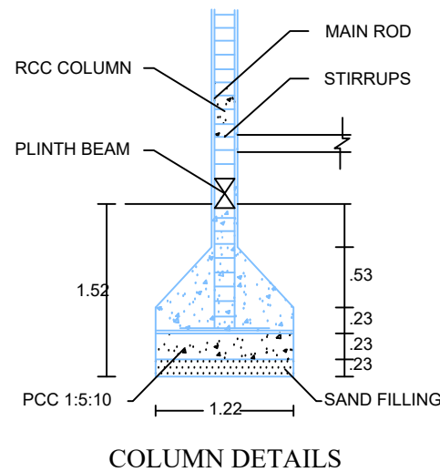
COLUMN DETAILS
