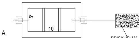
DETAILS OF RAIN WATER HARVESTING STRUCTURES (NOT TO SCALE)
