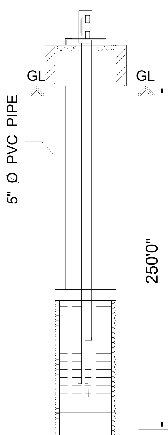
BOREWELL DETAILS
