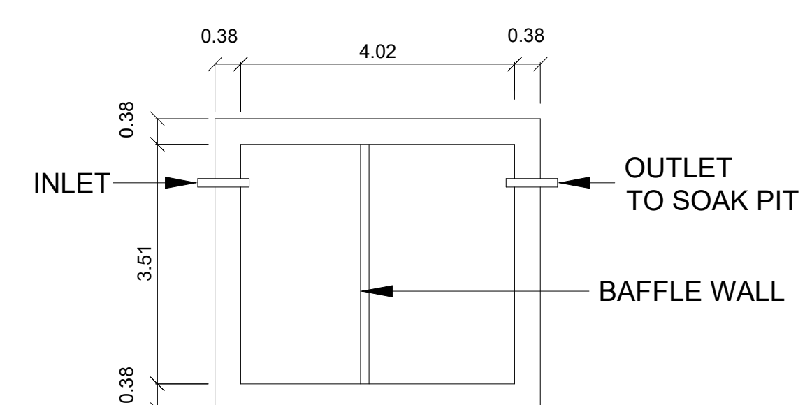
PLAN SEPTIC. TANK
