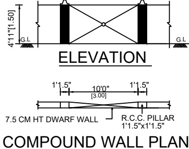
COMPOUND WALL PLAN
