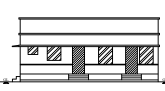
ELEVATION BLOCK - 2
