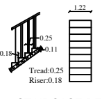
STAIRCASE DETAIL
