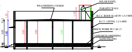
SECTION ON BB BLOCK - 2
