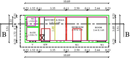
GROUND FLOOR PLAN BLOCK - 2
