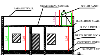
SECTION ON AA BLOCK - 1
