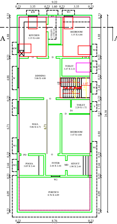
GROUND FLOOR PLAN BLOCK - 1
