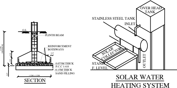
FOUNDATION DETAILS
