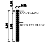
DETAILS OF PERCOLATION PIT
