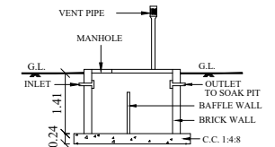
SECTION OF SEP.TANK
