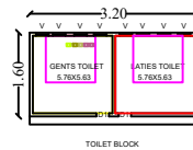
TOILET BLOCK
