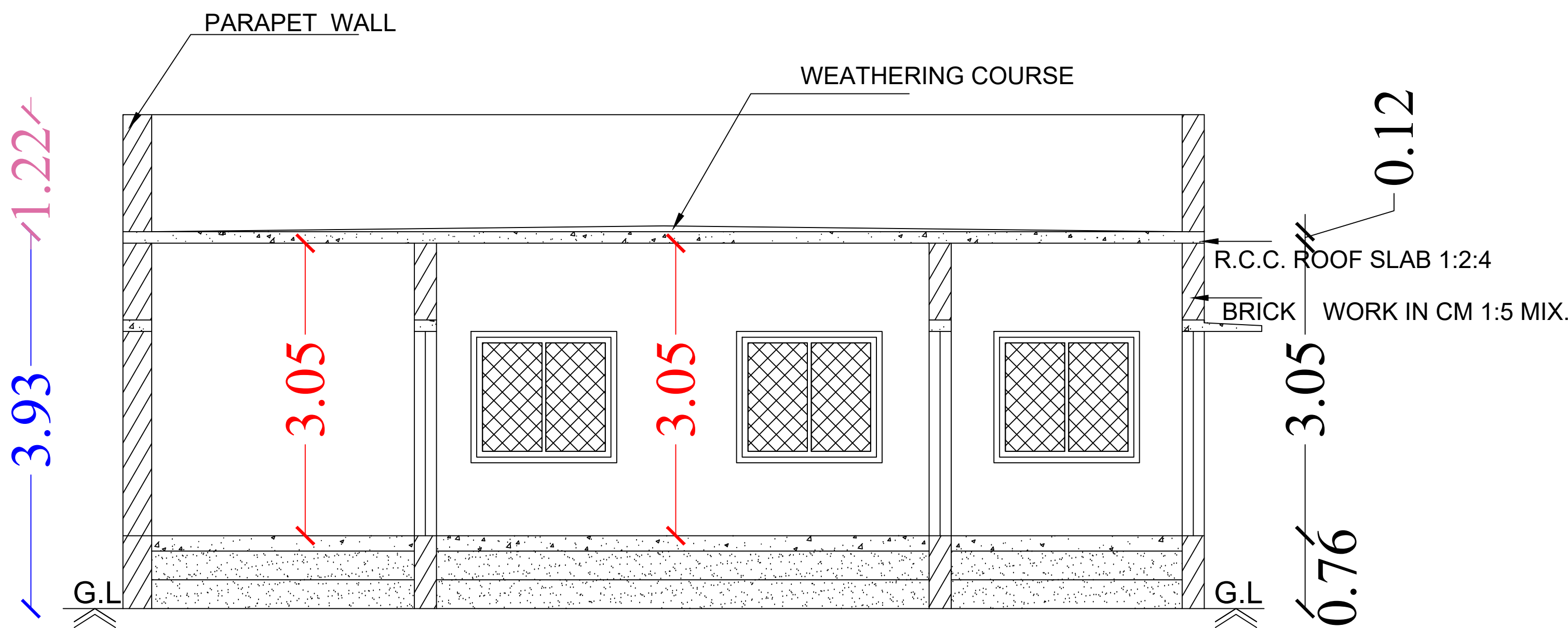
Section on-"AA"
