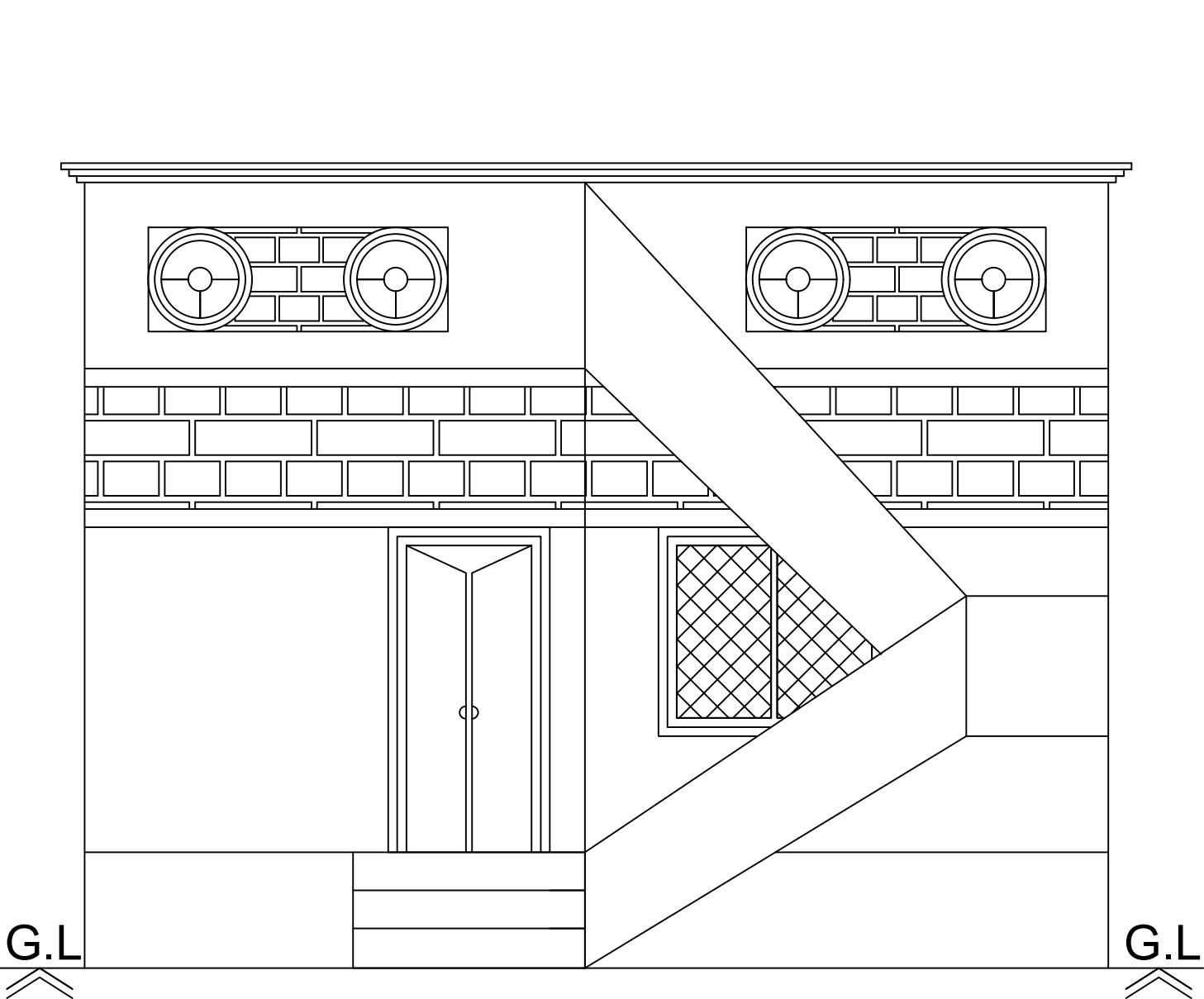
Front Elevation
