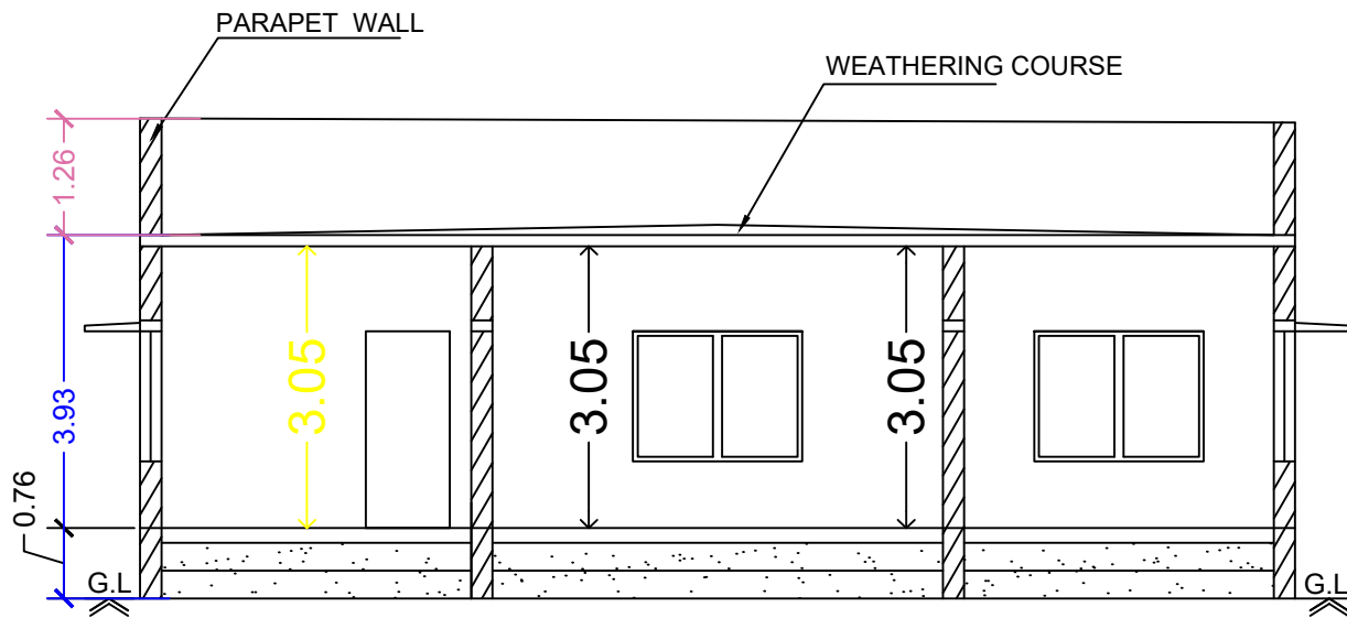
Section on-"AA"
