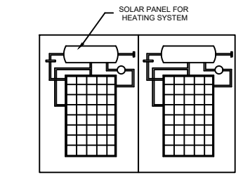
SOLAR HEATING SYSTEM
