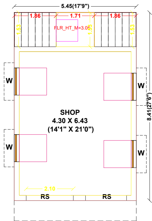
FLOOR-GROUND (COMMERCIAL )
