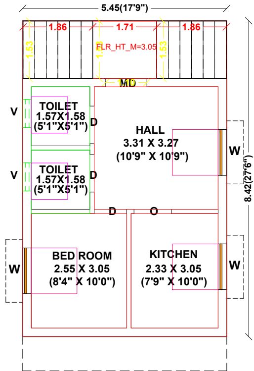
FLOOR-FIRST (RESIDENTIAL )
