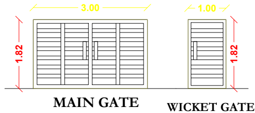
MAIN GATE WICKET GATE
