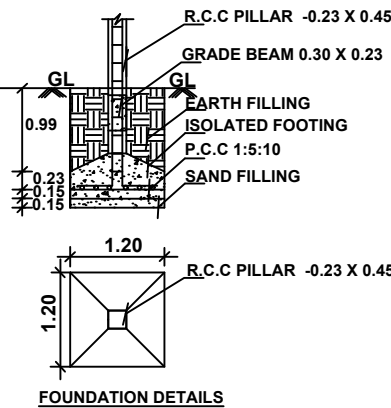
FOUNDATION DETAILS
