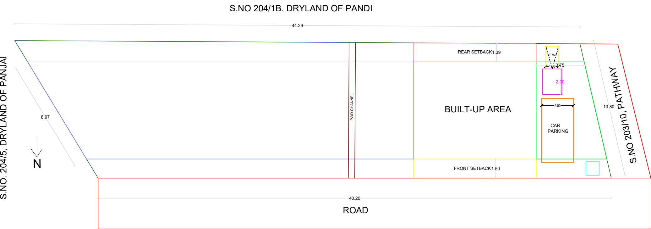
SITE PLAN
