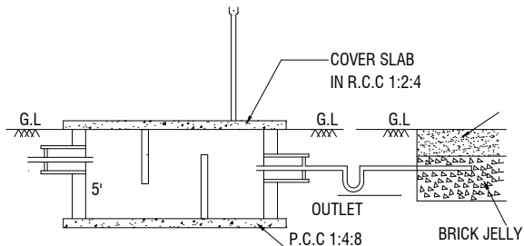
SECTION-AB
