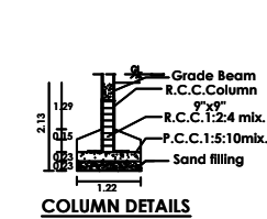
COLUMN DETAILS
