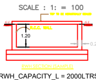
SCALE : 1: = 100 RW SECTION (SAMPLE) RW_CAPACITY_L = 2000LTRS
