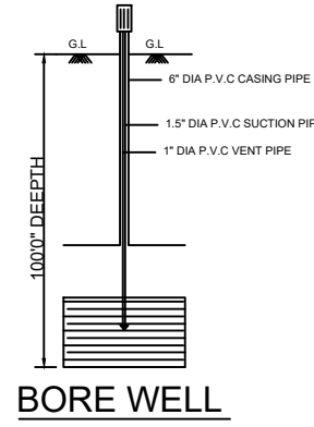
BORE WELL
