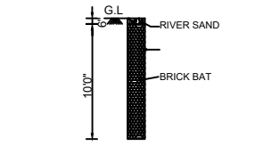
PERCOLATION PIT
