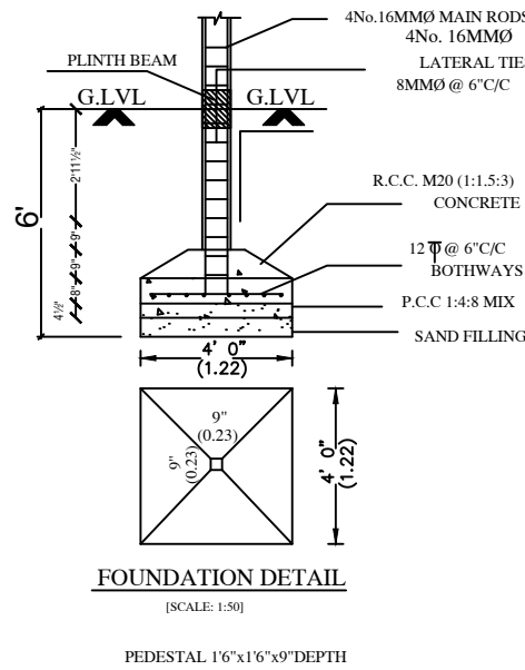
FOUNDATION DETAIL
