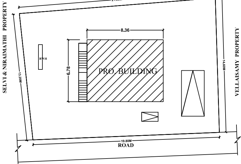
SITE PLAN
