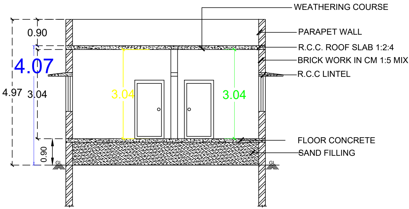
SECTION A1-A1
