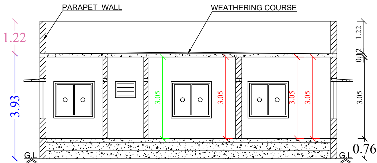
Section on-"AA"
