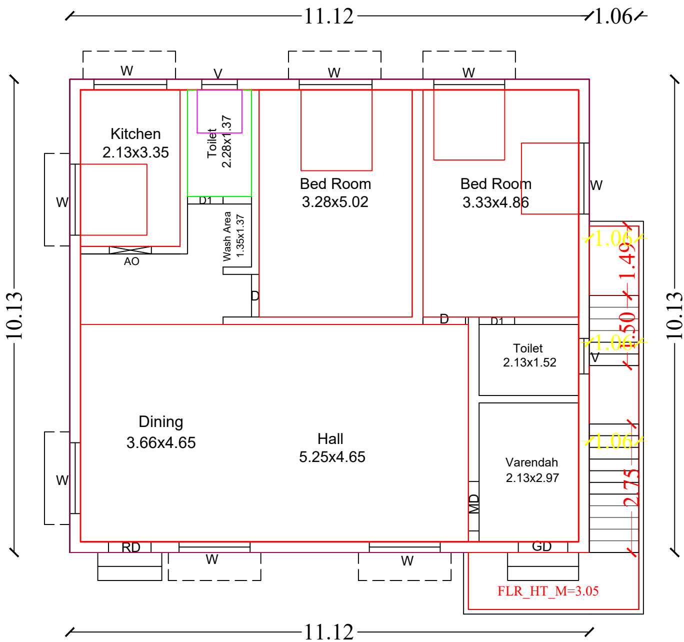
Ground Floor
