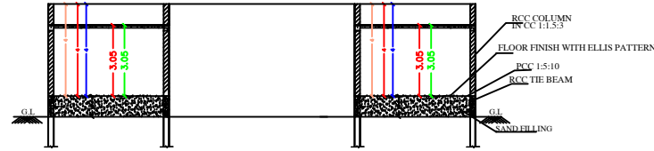
SECTION AA
