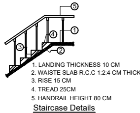
Staircase Details
