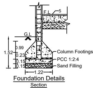
Foundation Details
