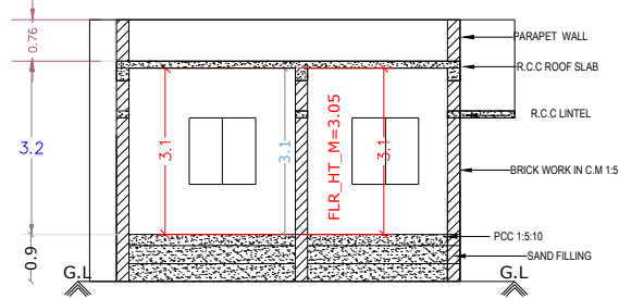
SECTION L-L
