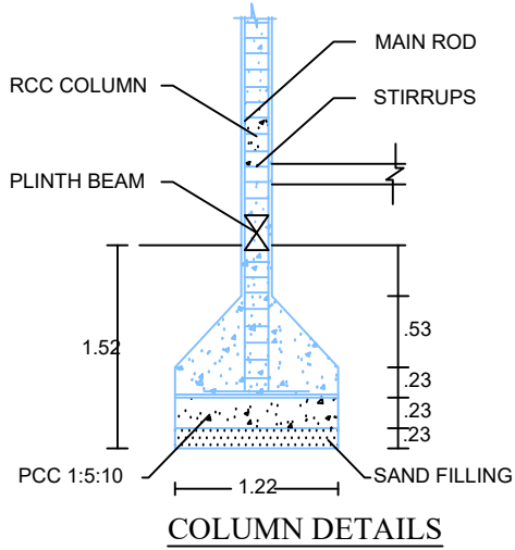
COLUMN DETAILS
