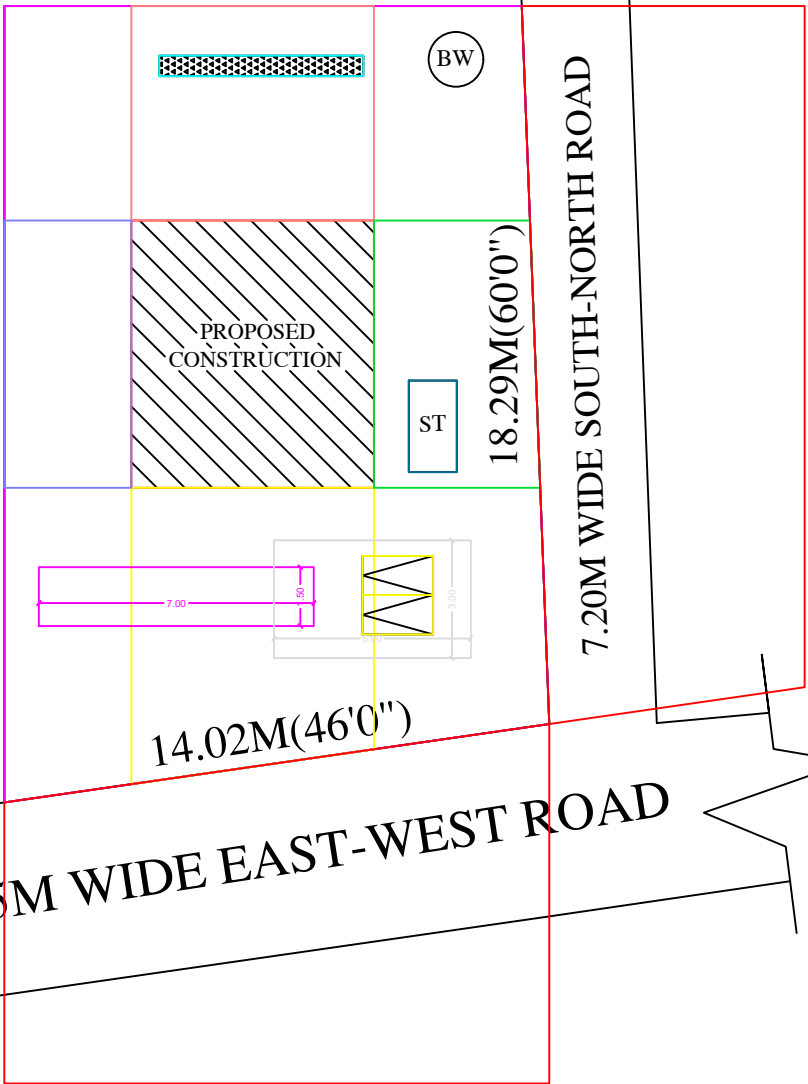
SITE PLAN
