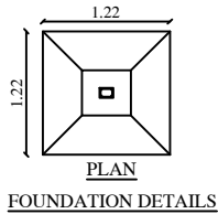
FOUNDATION DETAILS
