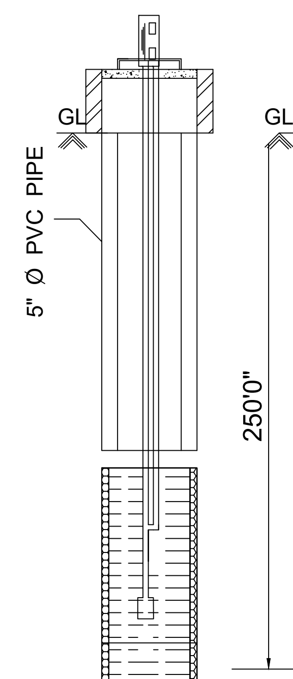
BOREWELL DETAILS
