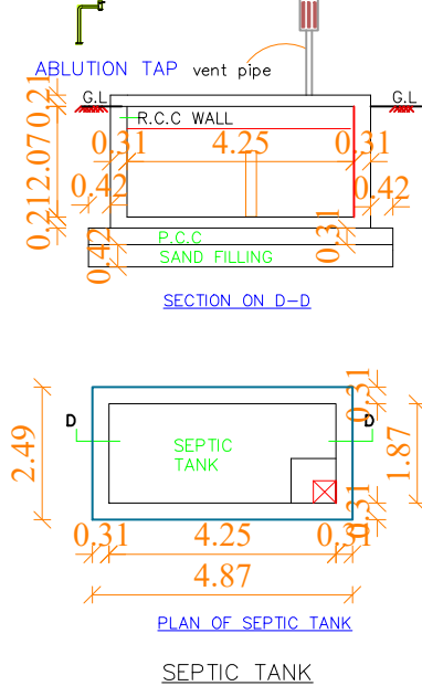
SEPTIC TANK
