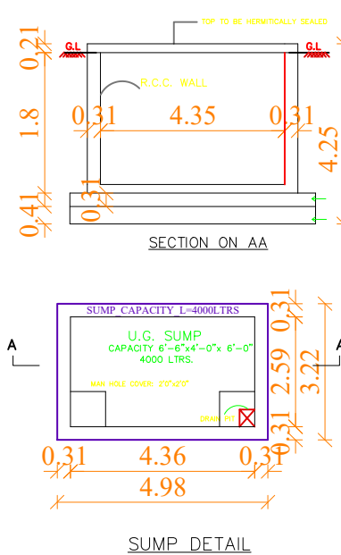
SUMP DETAIL
