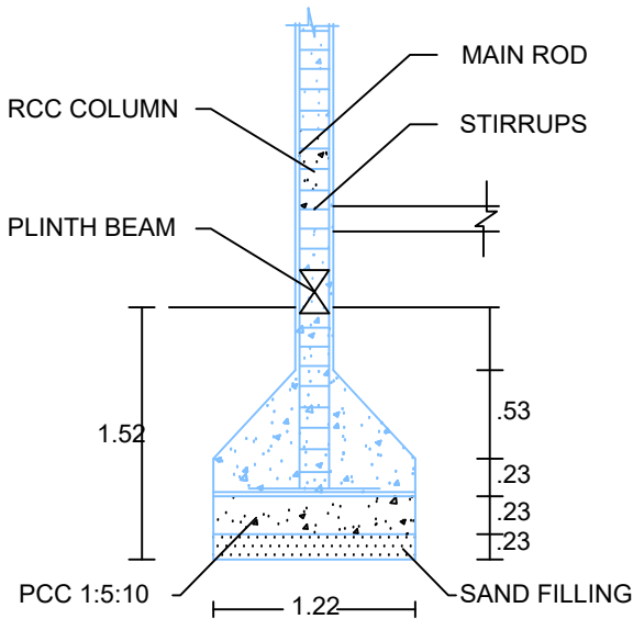
COLUMN DETAILS
