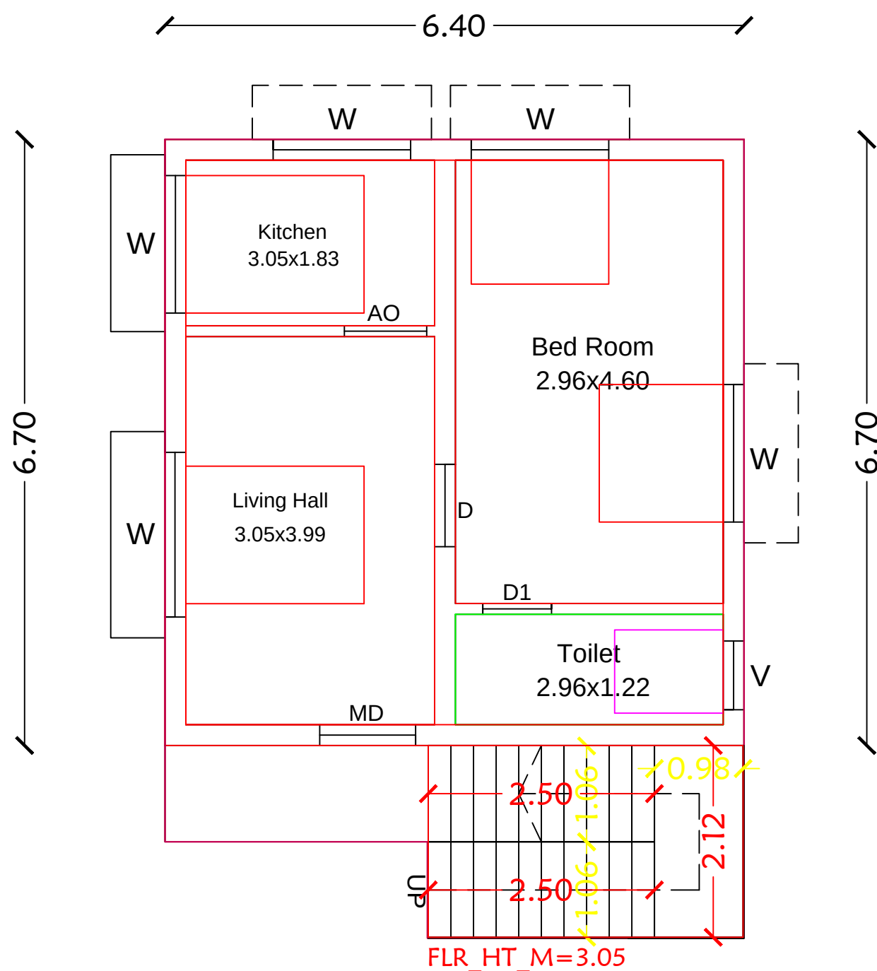
First Floor
