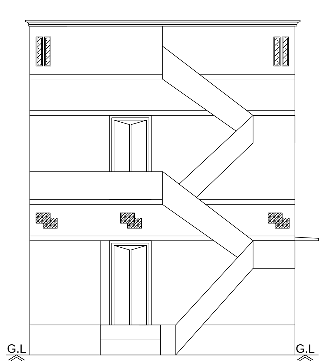
Front Elevation
