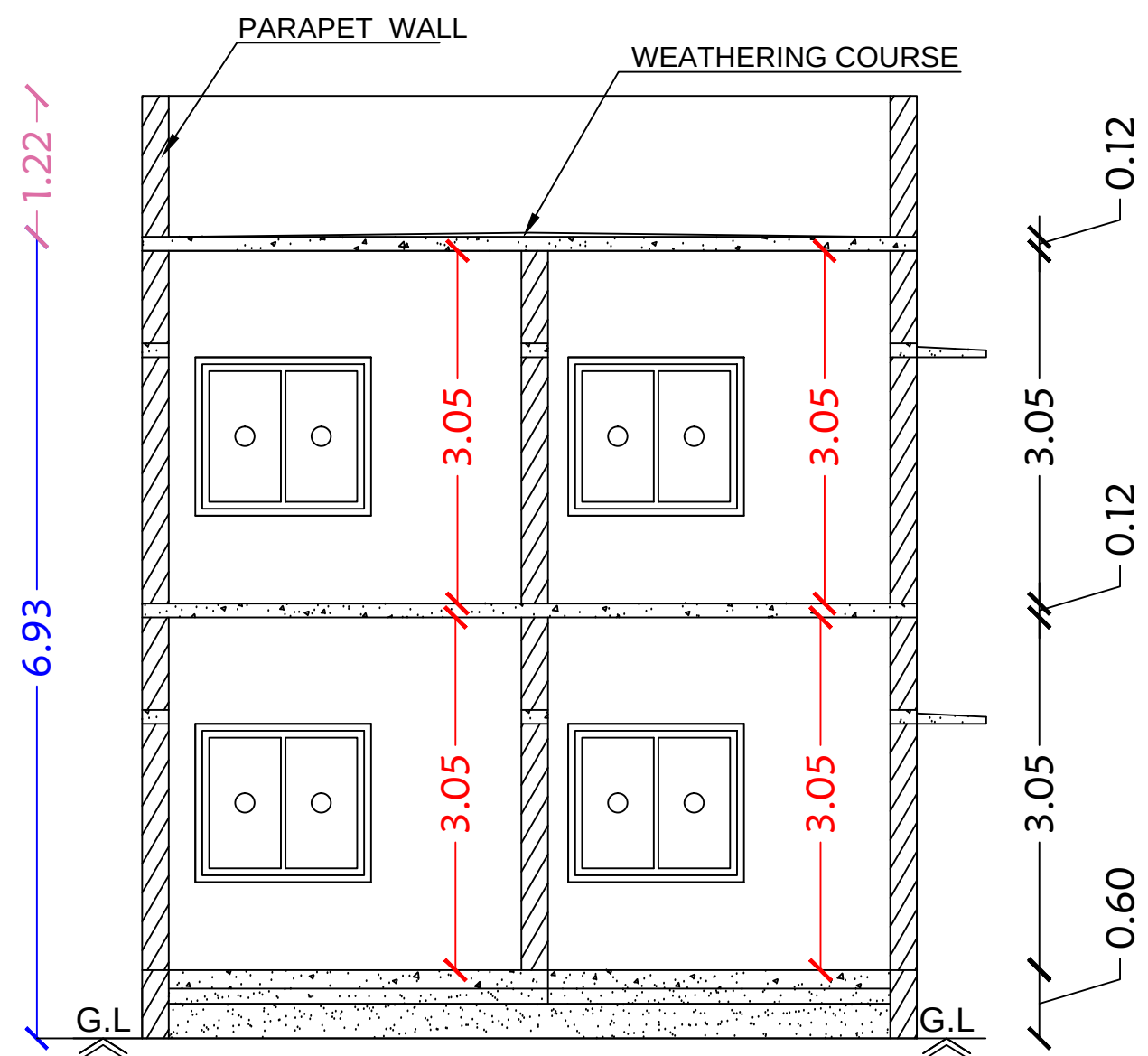
Section on-"AA"
