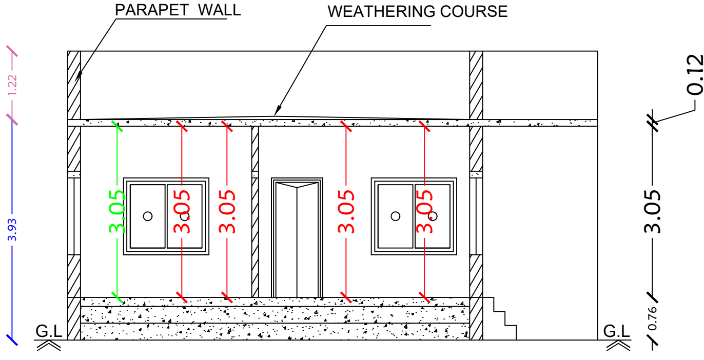
Section on-"AA"
