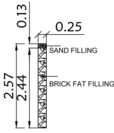
DETAILS OF PERCOLATION PIT
