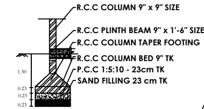
SECTION
