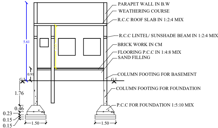
SECTION ON-AA
