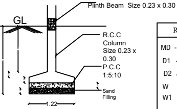
FOUNDATION DETAILS
