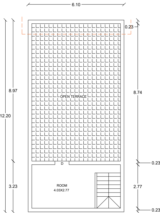
PRO FIRST FLOOR
