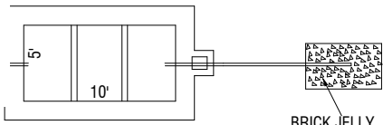
SEPTIC TANK & DISPERSION TRENCH DETAILS SCALE- 1:100
