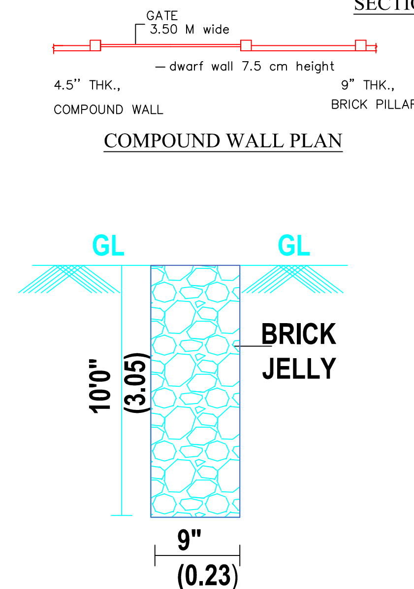
PERCULATION PIT
