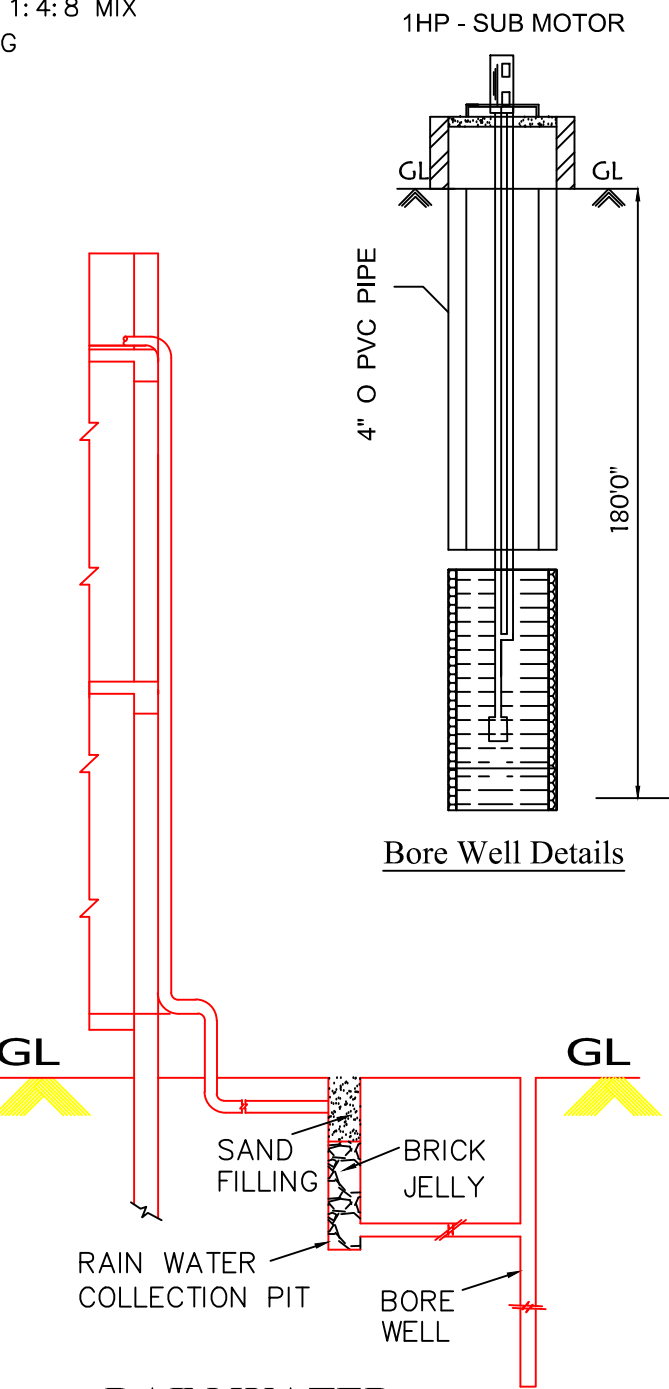
RAIN WATER HARVESTING SYSTEM
