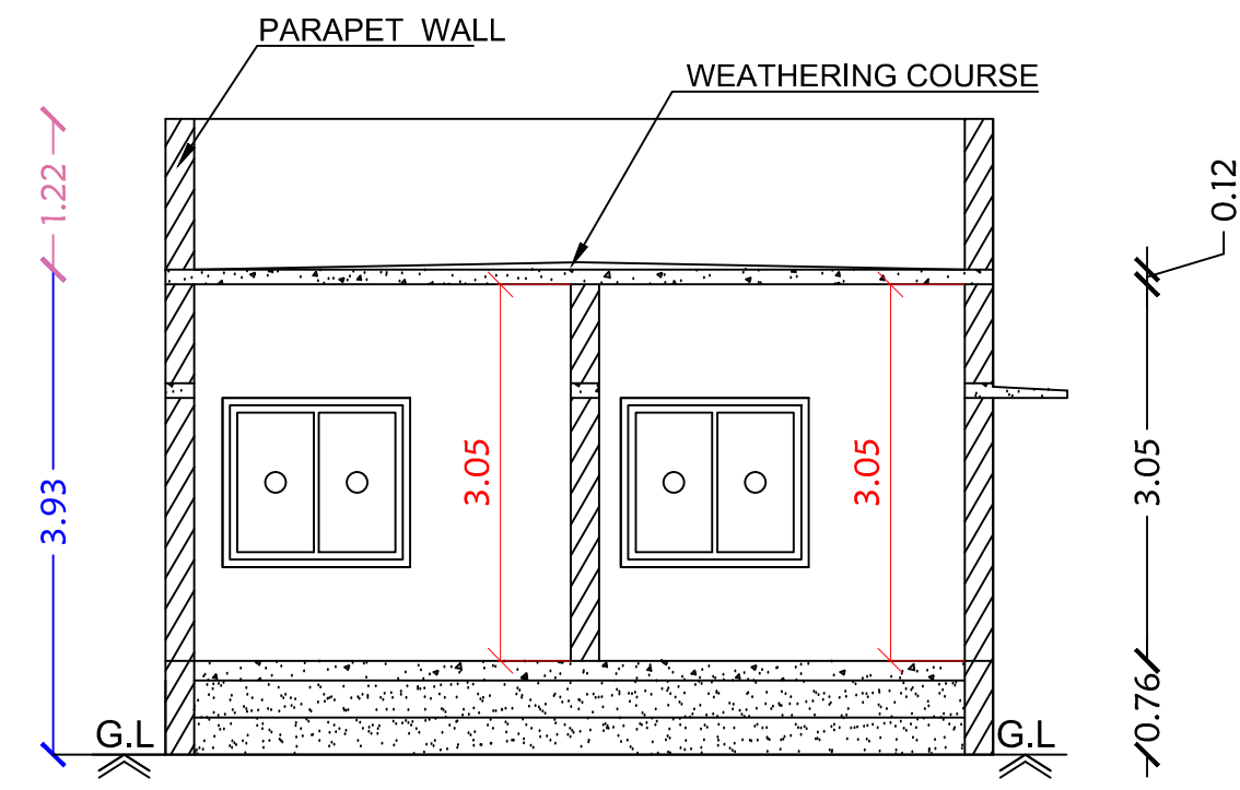
Section on-"AA"
