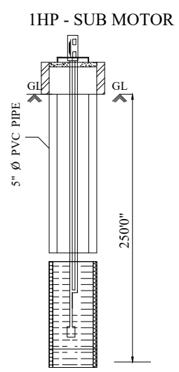
BOREWELL DETAILS
