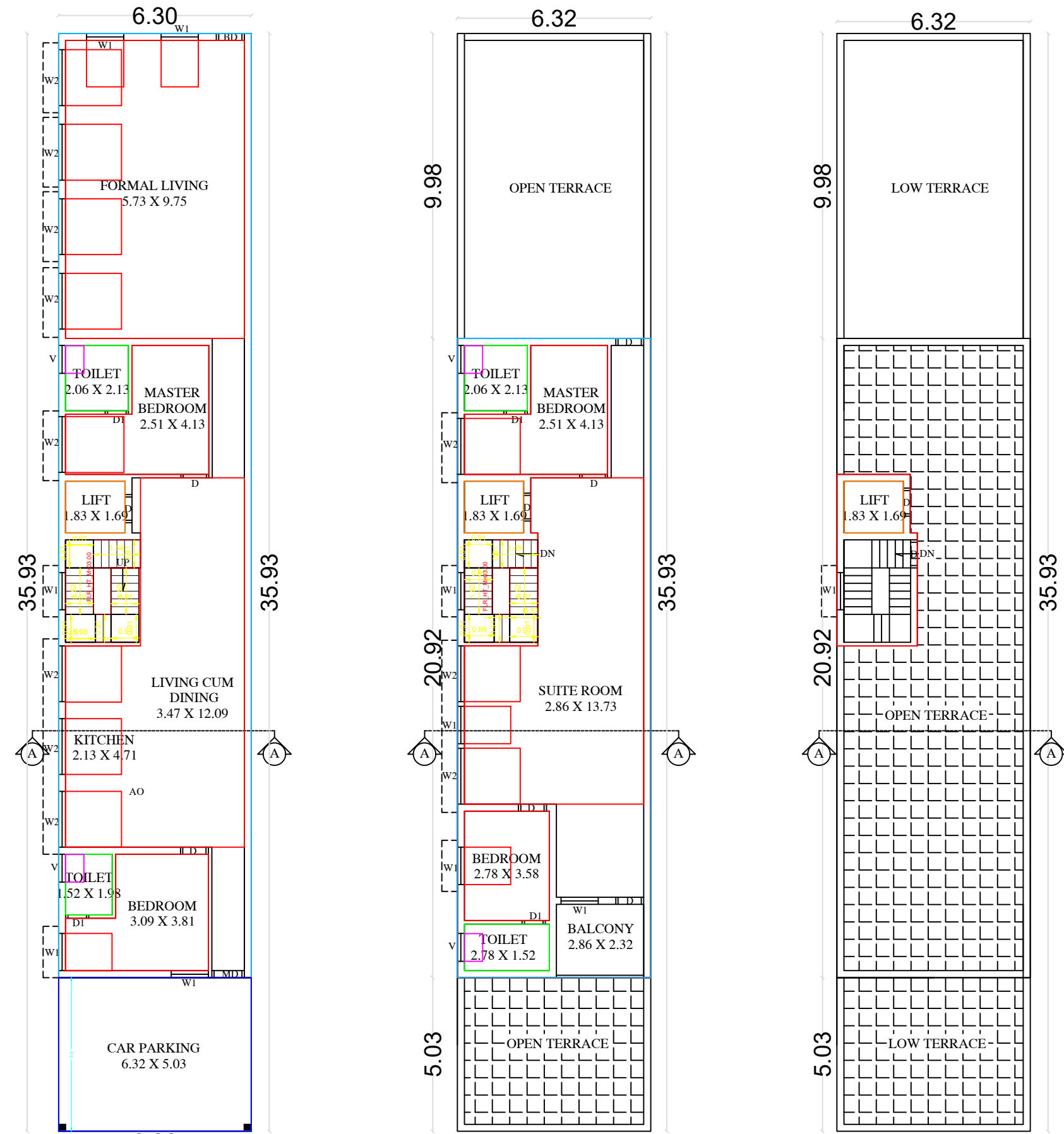
PROPOSED GROUND FLOOR PLAN PROPOSED FIRST FLOOR PLAN PROPOSED HEAD ROOM PLAN
