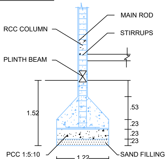
COLUMN DETAILS
