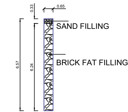
DETAILS OF PERCOLATION PIT
